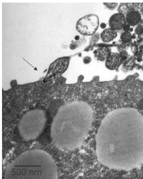
FIG. 5. Transmission electron micrograph of M. pneumoniae -infected hamster tracheal ring, demonstrating the close association of the attachment structure to the epithelium (arrow). (Copyright J. L. Jordan and D. C. Krause.)
