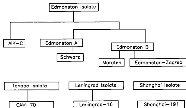
FIG. 4. Origin of selected strains of measles vaccine. Reprinted from reference 58 with permission.
